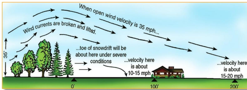
Figure 14 Diagram showing a windbreak and relationship between windbreak height and the subsequent impact on wind velocity (from: Tree Windbreaks for Farms and Homes , Purdue University Extension) presented by University of Arizona .
